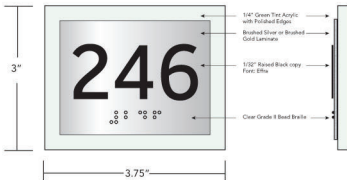
ROOM NUMBER PART# MAR21-1000
